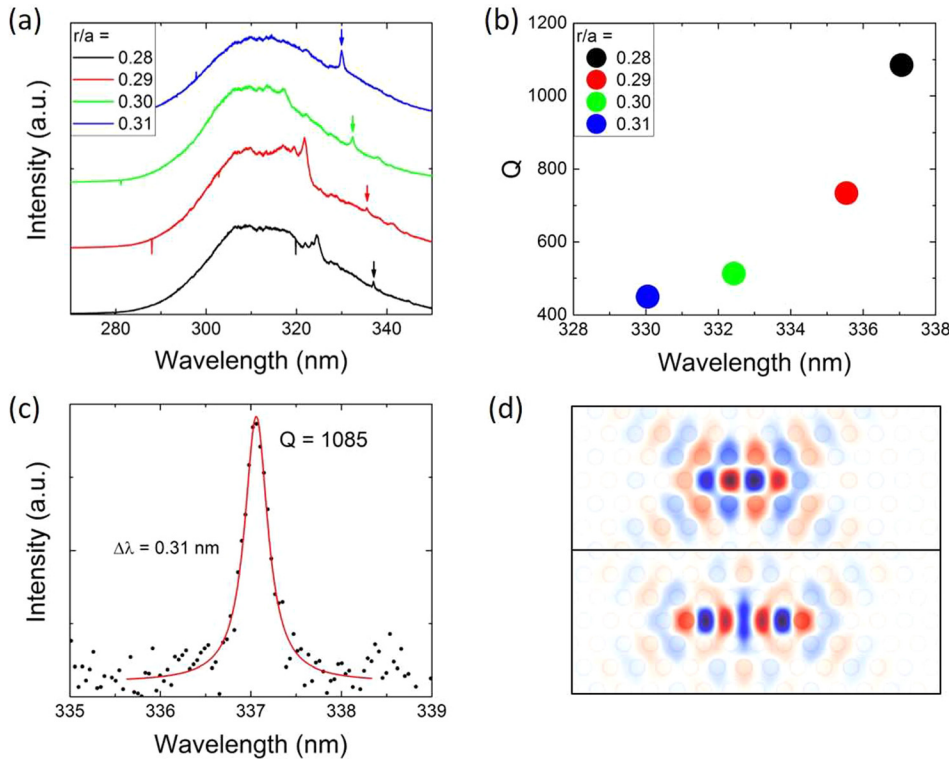
FIG. 2. L3 cavities with period a = 130 nm, hole displacement d/a = 0.15 , and nominal radii r/a = 0.28 to 0.31 . (a) \mu PL spectra for the different r/a moved along the y-axis for clarity. Arrows indicate fundamental modes. (b) Q factors for the fundamental modes in (a). (c) Measured spectrum (dots) and Lorentzian fit (line) of the fundamental mode of the L3 cavity with r/a = 0.28 shown in (a). (d) FDTD simulations of the Hz field of (top) the fundamental mode and (bottom) the first-order mode of an L3 cavity depicted in (a) with r/a = 0.28 .
