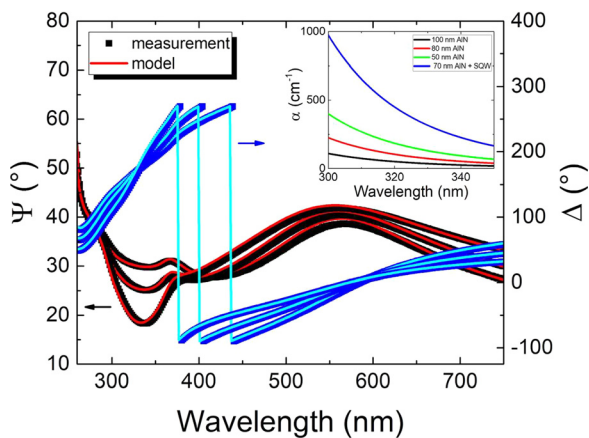
FIG. 4. Spectroscopic ellipsometry measurement (squares) and model (lines) for angles of incidence of 65^\circ , 70^\circ , and 75^\circ for a sample with 80 nm of AlN grown on Si (111). The inset shows the AlN absorption coefficient \alpha for samples with different AlN thicknesses.
