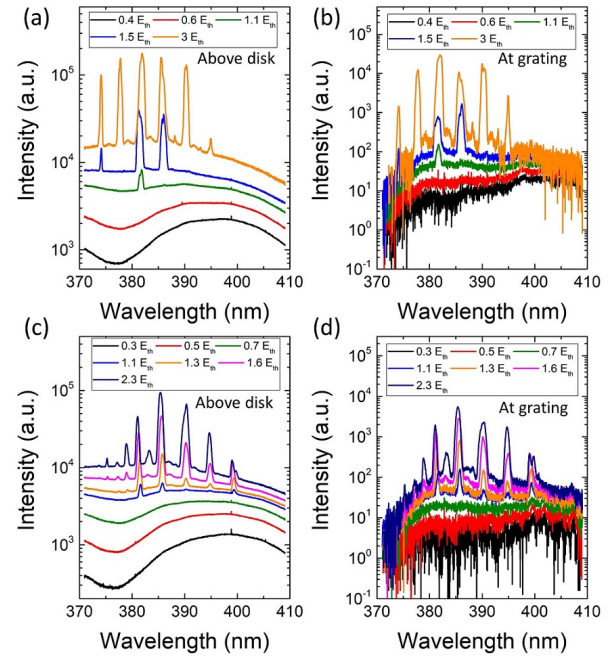
Fig. 3. Energy dependent pulsed optical pumping spectra of measured (a,c) above the disk and (c,d) at the grating coupler for devices with (a,b) a 50 nm gap and (c,d) an 90 nm gap. The thresholds are 0.18 \text{ mJ/cm}^2 per pulse for the 50 nm gap and 0.15 \text{ mJ/cm}^2 per pulse for the 90 nm gap.
