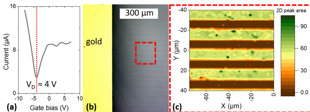
FIG. 2. Graphene as an infrared transparent, work function tunable electrode. (a) Transfer curve (drain current as a function of the gate bias) for a graphene layer used as a channel of a field-effect transistor with a gate made of \text{LaF}_3 ionic glass. (b) Image of the patterned graphene deposited onto a \text{LaF}_3 substrate and connected to a gold contact. (c) Map of the intensity of the graphene in the 2D Raman mode of graphene for the electrode deposited on \text{LaF}_3 . On this map, the substrate is brown while the graphene is yellow-green.
