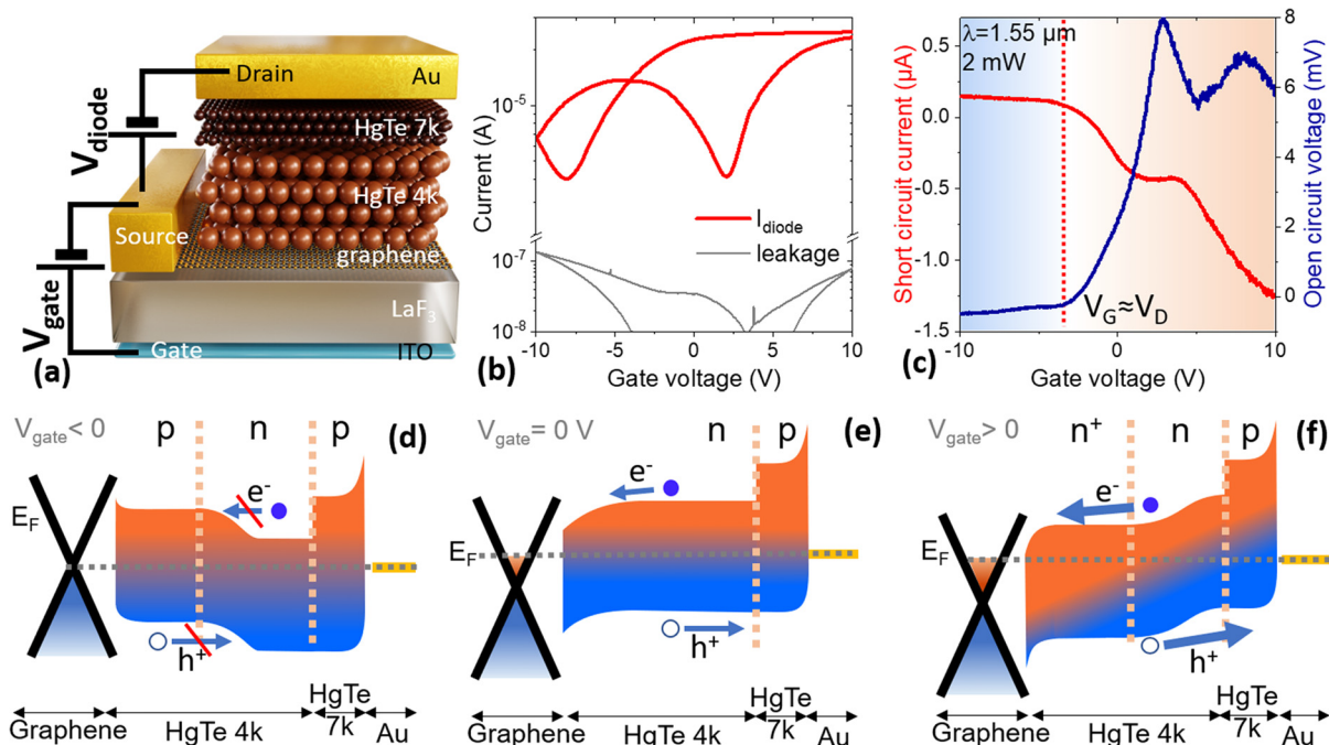
FIG. 3. Gate tunable vertical geometry infrared diode. (a) Sketch of the gate tunable diode based on the ITO/ \text{LaF}_3 /graphene/HgTe4 k/HgTe7 k/gold stack. (b) Current through the diode while the gate bias is tuned ( V_{\text{diode}} = 0.1 \text{ V} ). (c) Short circuit current and open circuit voltage for the diode under illumination ( \lambda = 1.55 \mu\text{m} – P = 2 \text{ mW} ) as a function of gate bias. Band structure of the diode under negative gate bias (part d), 0 V bias (part e), and positive gate bias (part f). Measurements are conducted at 220 K.
