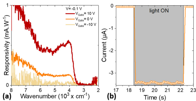
FIG. 4. Infrared detection using the gate tunable diode. (a) Spectral response of the gate tunable diode operated under three gate biases, while the diode bias is set to -0.1 V. Curves have been normalized to take into account the amplifier gain. (b) Photocurrent under 0 V diode bias and 10 V gate bias while the illumination ( \lambda = 1.55 \mu\text{m} , P = 2 mW) is turned on and off. Measurements are conducted at 220 K.
