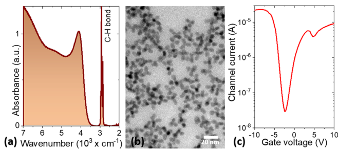
FIG. 1. HgTe infrared nanocrystals. (a) Absorption spectrum of the HgTe NCs. (b) Transmission electronic microscopy image of HgTe NCs associated with the spectrum of part (a). (c) Transfer curve (drain current as a function of the gate bias) for a thin film of HgTe NCs used as the channel of a field-effect transistor whose gate is made of \text{LaF}_3 ionic glass.
