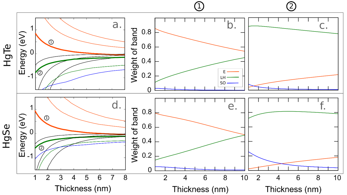
Figure S 11 Calculated subbands of HgSe and HgTe quantum wells. Energy of HgTe subbands (a) and band composition of the subbands labeled as ① (b) and ② (c), as a function of the quantum well thickness. (d-f): same but for HgSe.
